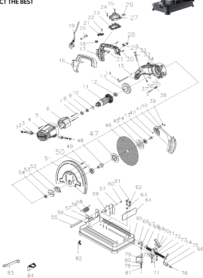
KI CM355 CUT-OFF MACHINE
